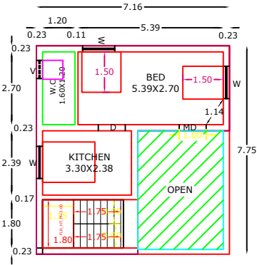
PRO FIRST FLOOR RESIDENTIAL PLAN
