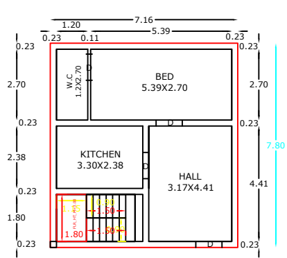
EXT GROUND FLOOR RESIDENTIAL PLAN
