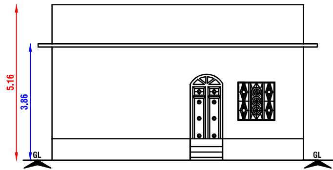
FRONT ELEVATION
