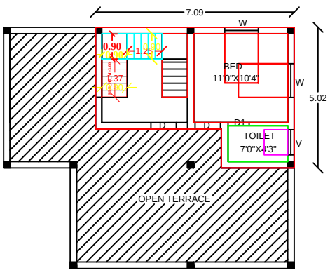
PRO.FIRST FLOOR PLAN
