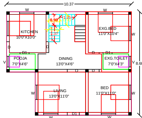
EXG.& PRO.GROUND FLOOR PLAN
