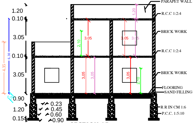
SECTION AB
