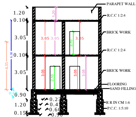
SECTION AB
