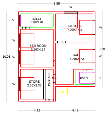
PROPOSED G.FLOOR PLAN
