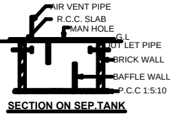
SECTION ON SEPTIC TANK
