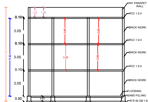
SECTION AB
