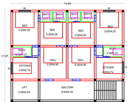
SEC.FLOOR PLAN
