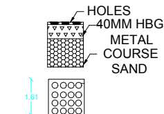
RWH_CAPACITY_L = 2000LTRS RAIN WATER COLLECTING TANK
