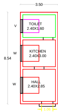
GROUND FLOOR
