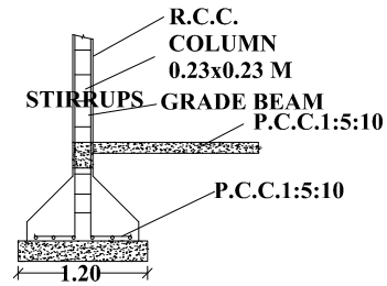
COLUMN DETAIL
