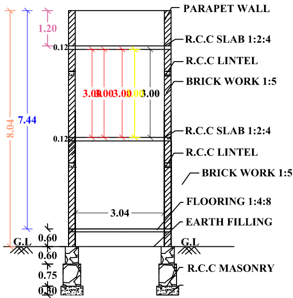
"SECTION "AB"
