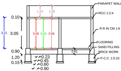
SECTION AB
