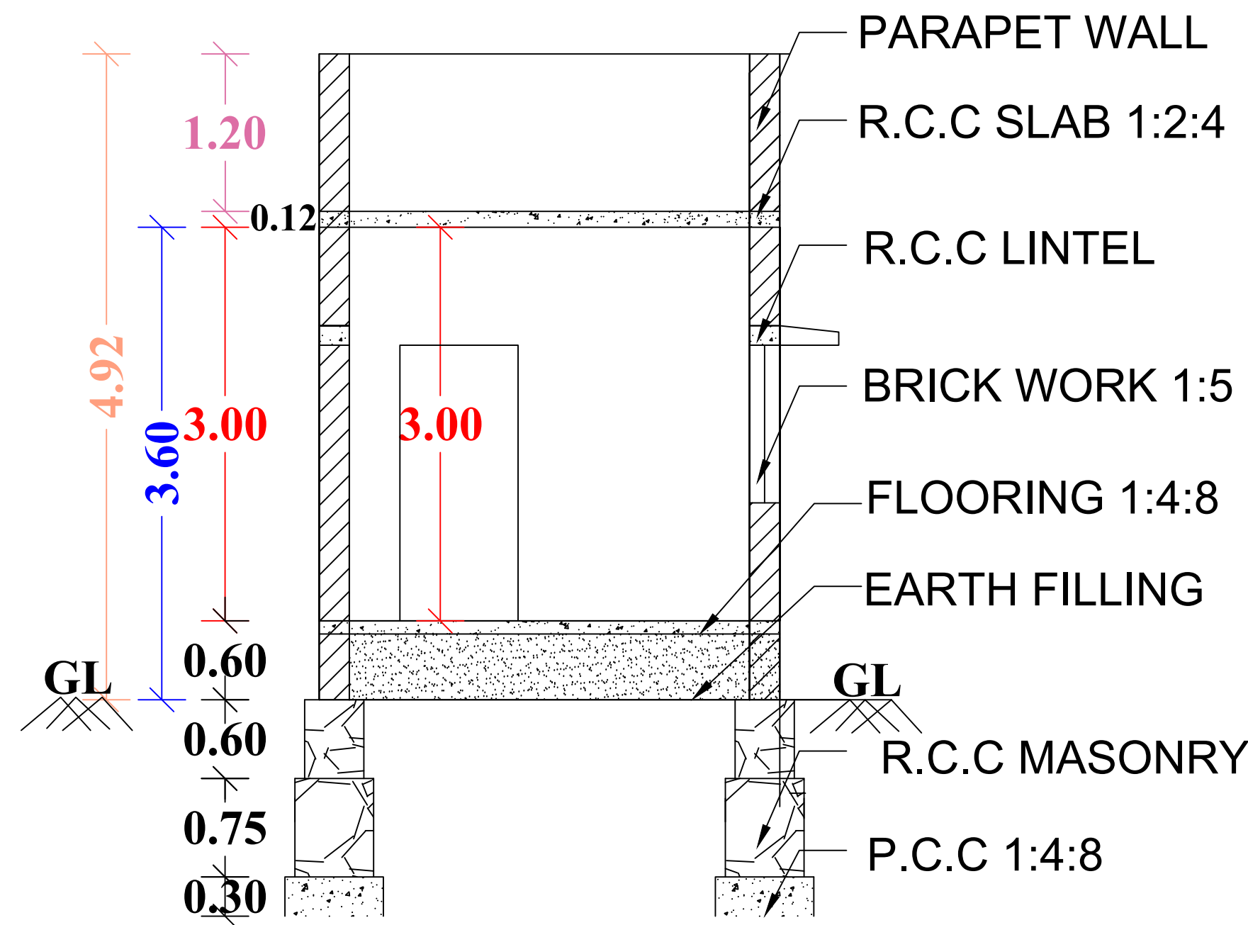
"SECTION "AB"
