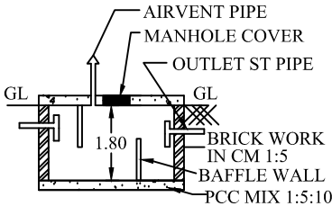
SECTION ON SEPTICTANK
