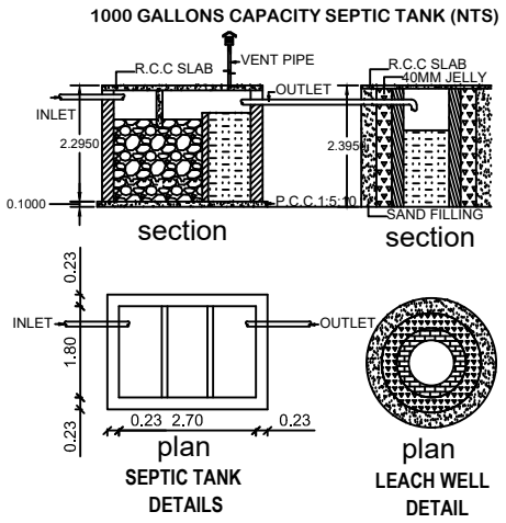
1000 GALLONS CAPACITY SEPTIC TANK (NTS)
