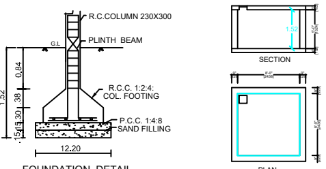
FOUNDATION DETAIL
