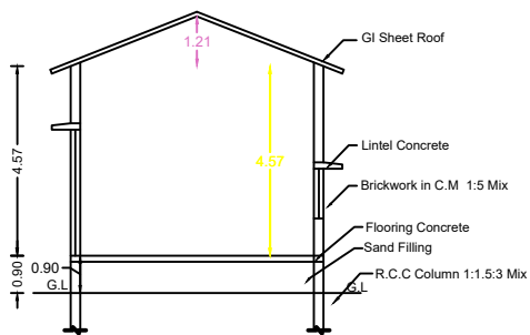
SECTION ON "RK"
