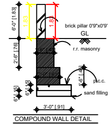
COMPOUND WALL DETAIL scale: 01" = 40"
