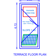
TERRACE FLOOR PLAN
