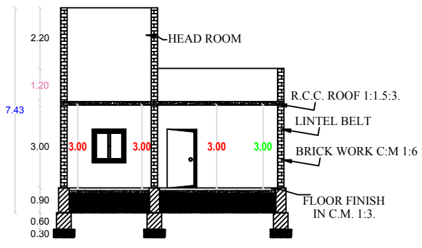
SECTION "AB"
