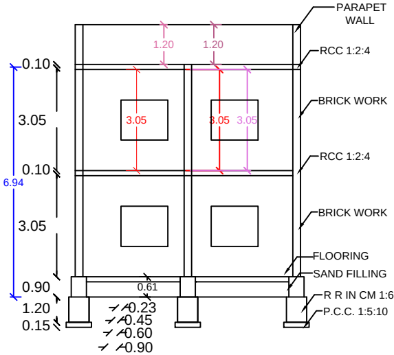
SECTION AB
