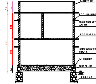
SECTION ON A-A & A'-A'
