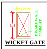
WICKET GATE
