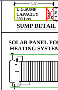
RAIN WATER HARVESTING
