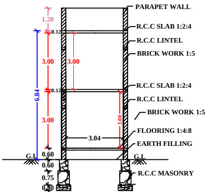
"SECTION 'AB'"
