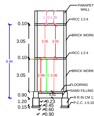
SECTION AB
