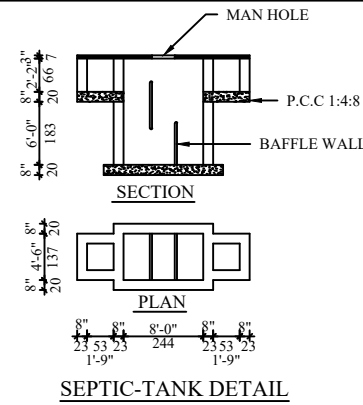
SEPTIC-TANK DETAIL
