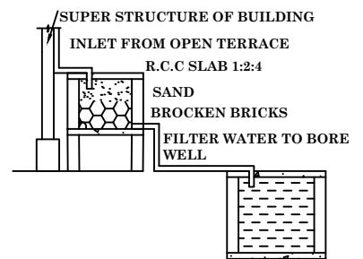
DETAILS OF FILTER BED & WELL
