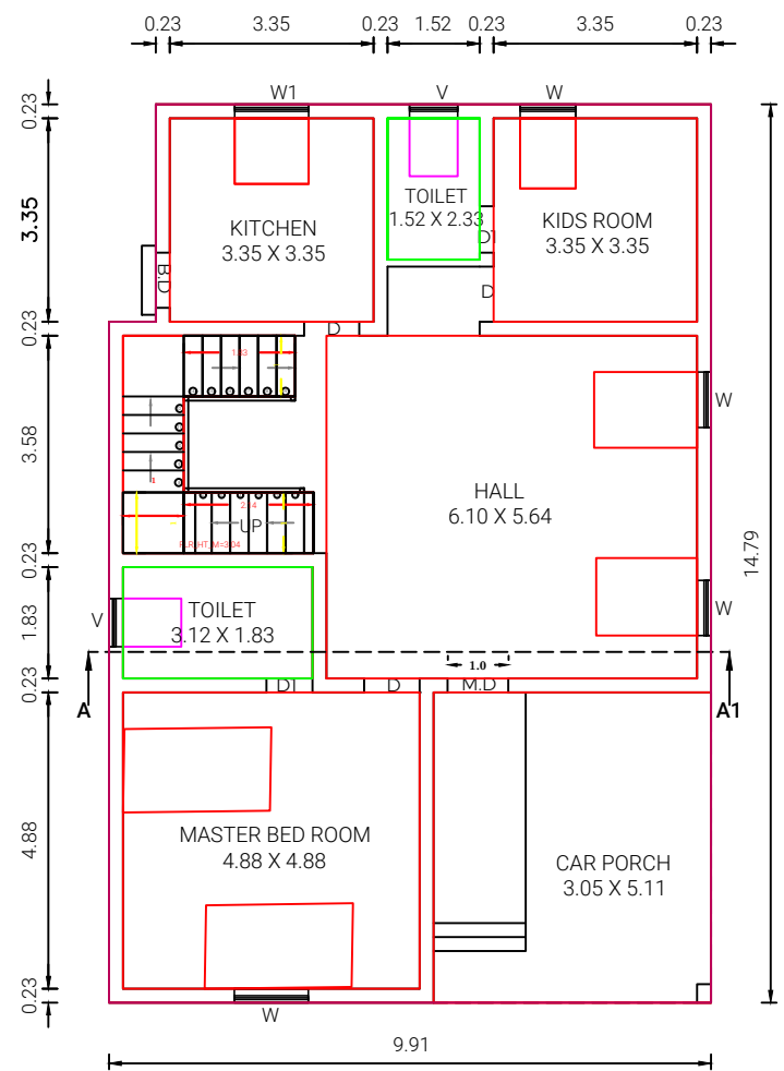
PLAN - GROUND FLOOR
