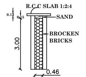
PERCOLATION PIT
