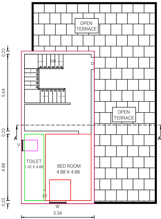
PLAN - FIRST FLOOR (PROPOSED)
