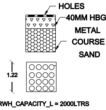
RAIN WATER COLLECTING TANK
