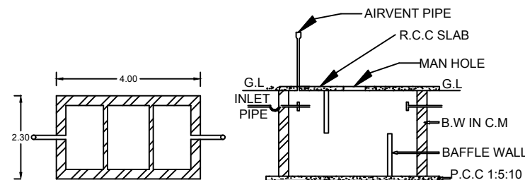
RAIN WATER HARVESTING SYSTEM
