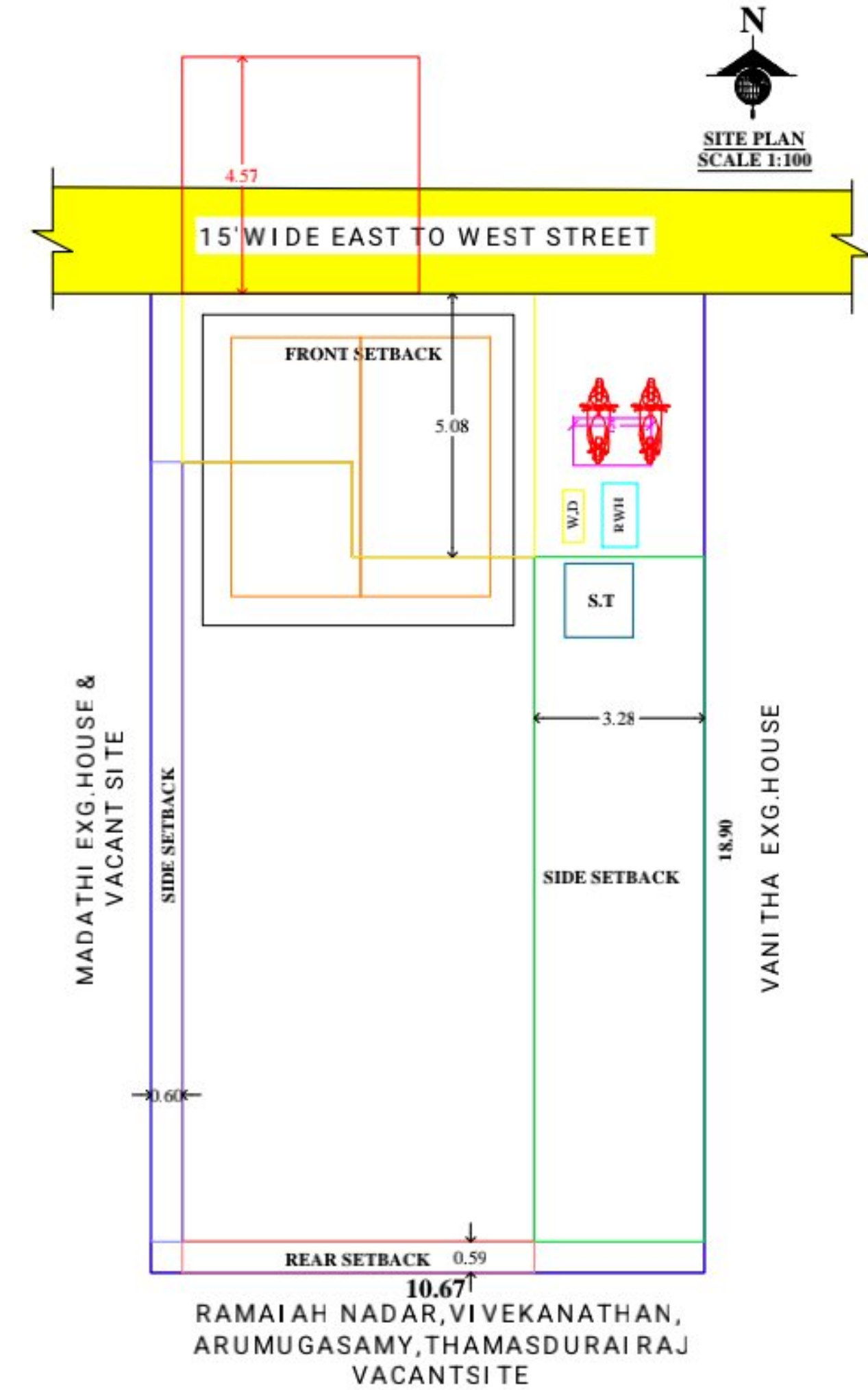
SITE PLAN
