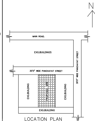
LOCATION PLAN
