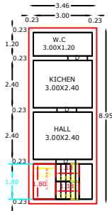
EXT GROUND FLOOR RESIDENTIAL PLAN
