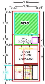
PRO FIRST FLOOR RESIDENTIAL PLAN
