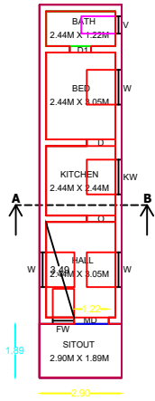
TYPICAL_FLOOR_PLAN=1
