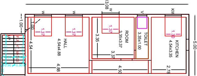
PROPOSED GROUND FLOOR PLAN
