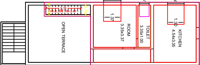
PROPOSED FIRST FLOOR PLAN
