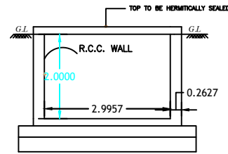
RWH SECTION
