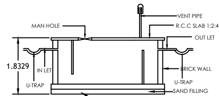
SECTION E-F SEPTIC TANK DETAIL
