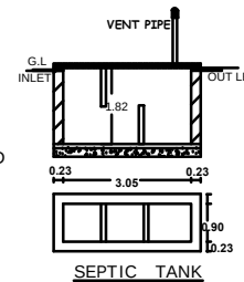
SEPTIC TANK DETAILS
