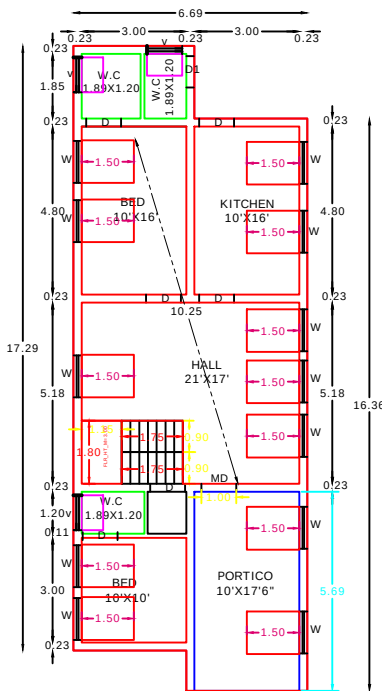
EXTG GROUND FLOOR PLAN
