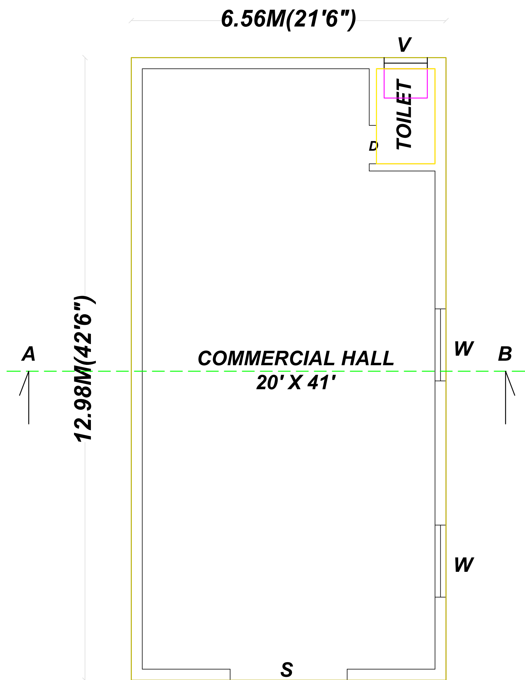
PLAN
