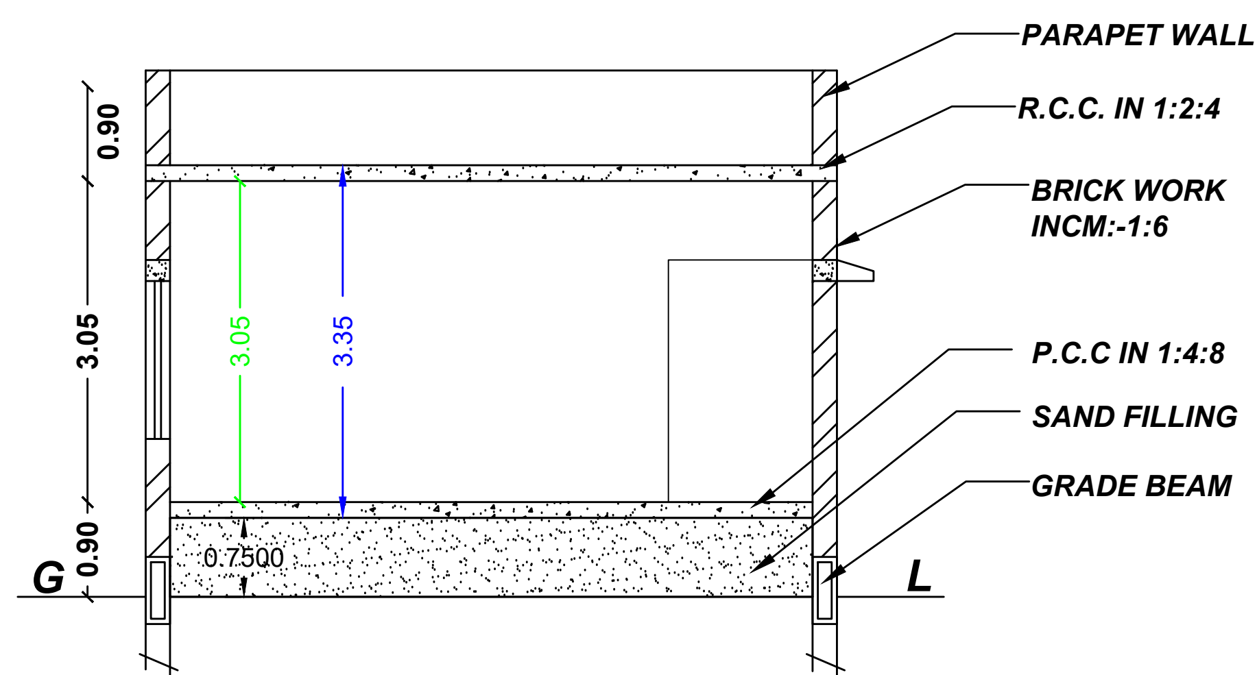
SECTION "AB"
