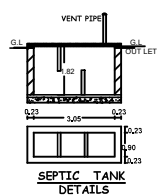
SEPTIC TANK DETAILS
