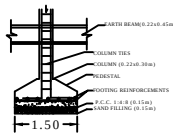
FOUNDATION DETAILS
