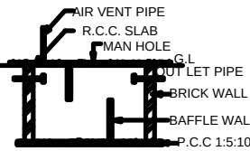
SECTION ON SEPT. TANK
