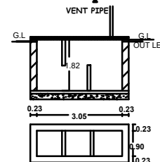
SEPTIC TANK DETAILS
