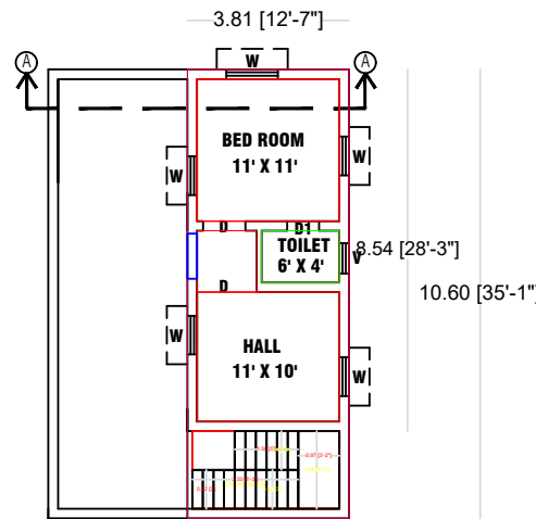
RST FLOOR PLAN
