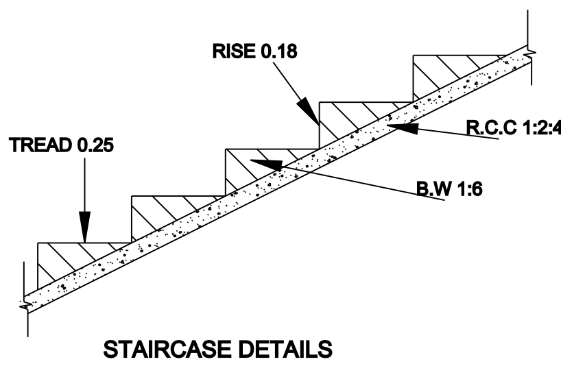
STAIRCASE DETAILS
