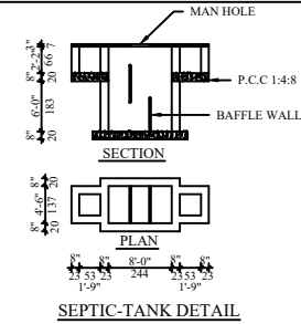
SEPTIC-TANK DETAIL
