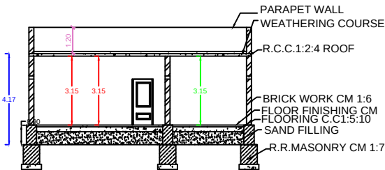
SECTION ON SV
