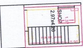
PRO FIRST FLOOR PLAN
