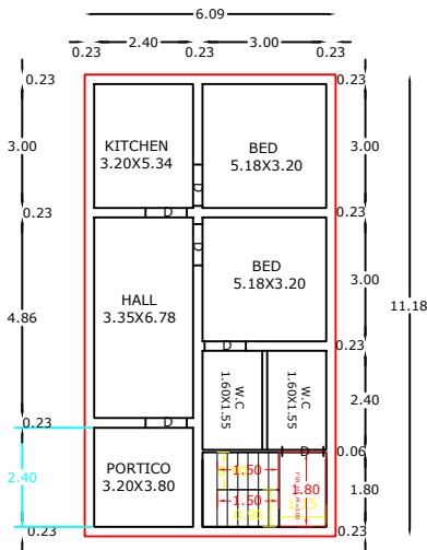
EXT GROUND FLOOR RESIDENTIAL PLAN
