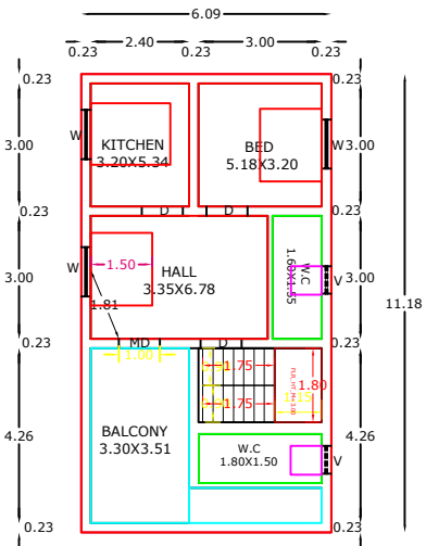
PRO FIRST FLOOR RESIDENTIAL PLAN
