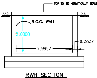
RWH SECTION
