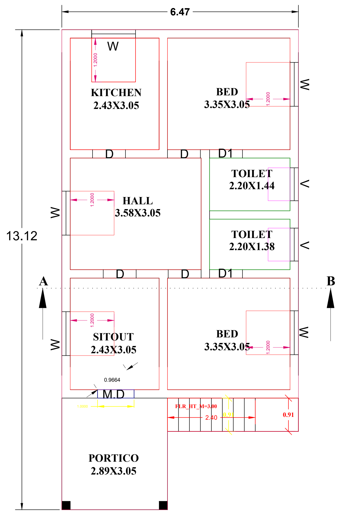
PLAN
