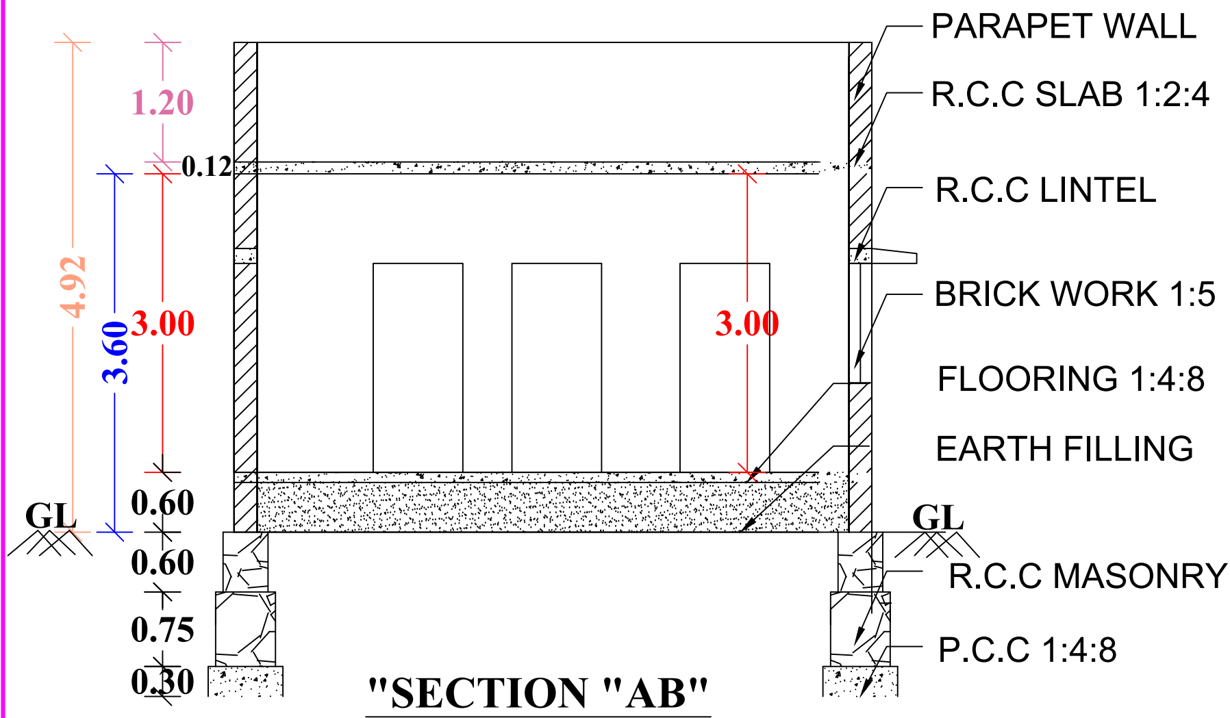
"SECTION "AB"
