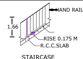
STAIRCASE
