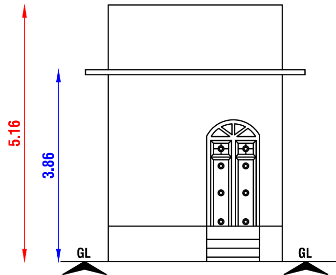
FRONT ELEVATION
