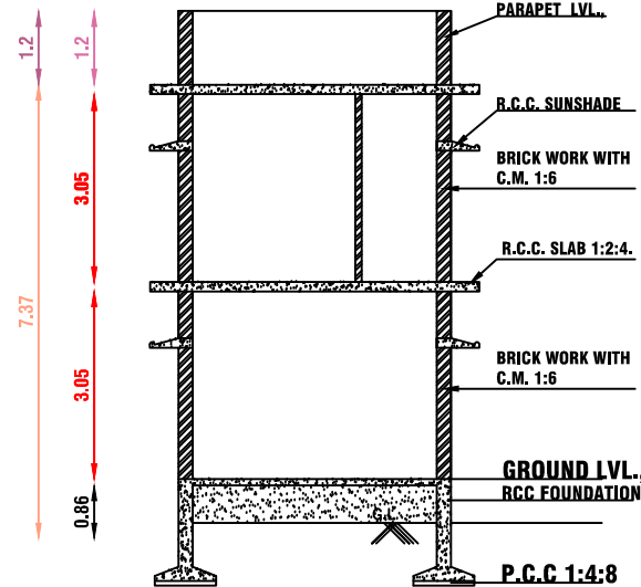
SECTION ON A-A & A'-A'
