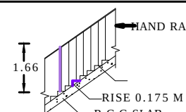
STAIRCASE
