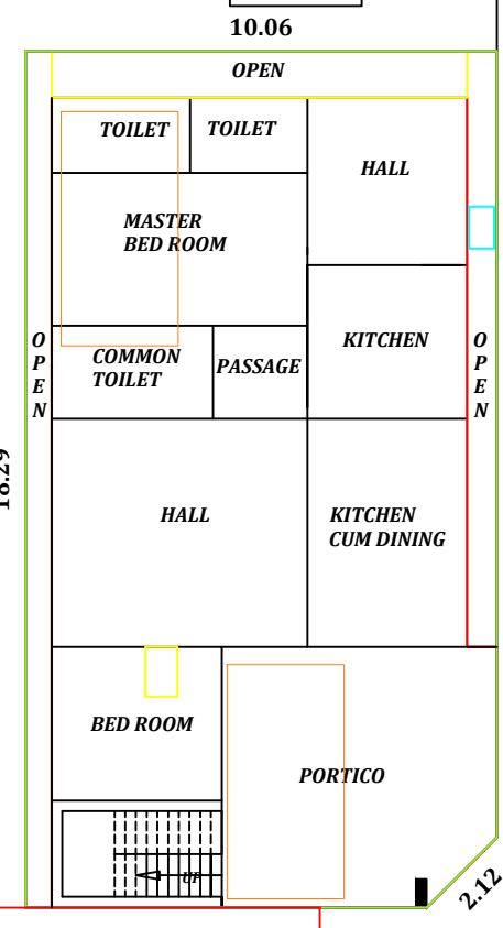
SITE PLAN
