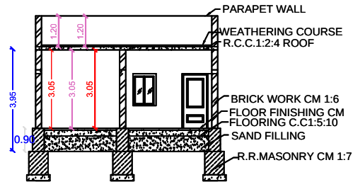
SECTION ON SV
